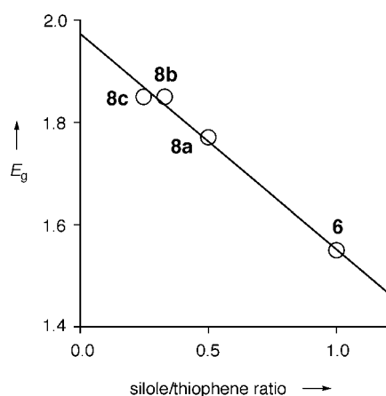
Figure 2. Plot of the band gaps ( E_g ) determined from absorption edge versus silole/thiophene ratios for a series of silole-thiophene copolymers.
